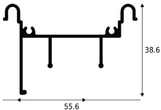
PF5-JL16 0.485 KG/M
