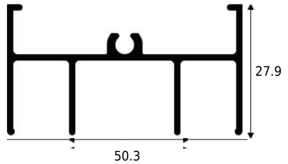
MB-002 0.505 KG/M
