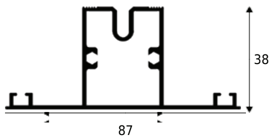
MAN-008 0.960 KG/M
