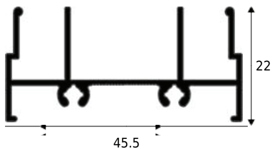
KDK-005 0.358 KG/M
