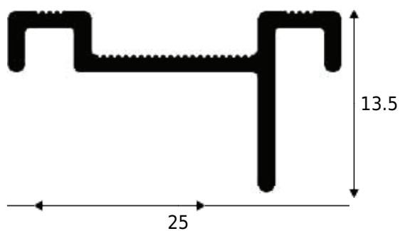
PF5-BL16
