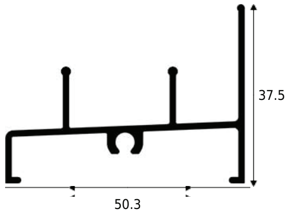
MB-001 0.460 KG/M
